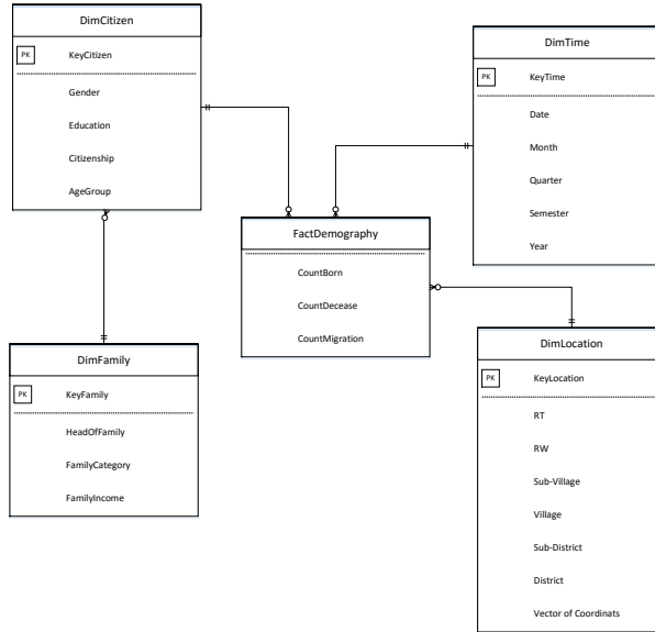
Figure 7. Data Warehouse Design for Demography
