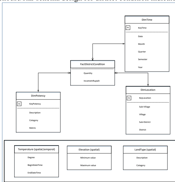
Figure 6. Data Warehouse Design for District Condition
