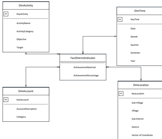
Figure 8. Data Warehouse Design for District Performance Indicator
