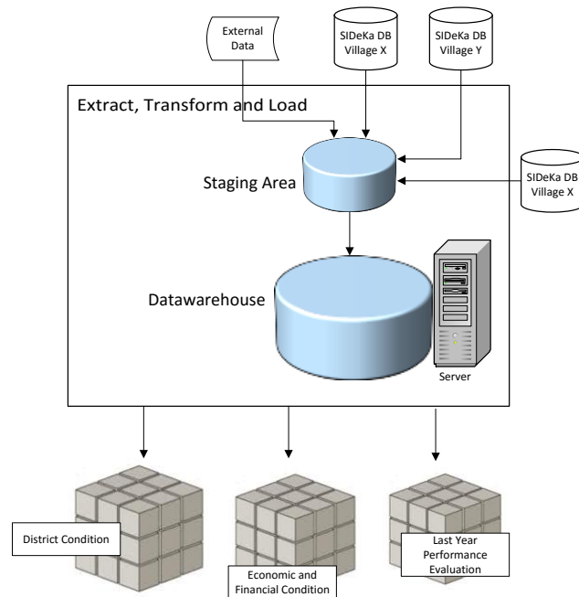
Figure 5. Supra Village OLAP Business Intelligence Application Architecture
