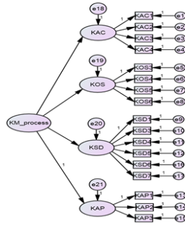
Fig. 2: Second-order CFA
