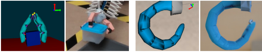
(a) Simulation of the soft grasper described in [72] (left). Grasper of Flexo (right). Comparison between simulated (right) and real. (b) Simulation (left) of octopus tentacle based on a similar design as described in [72] and real prototype (right).
