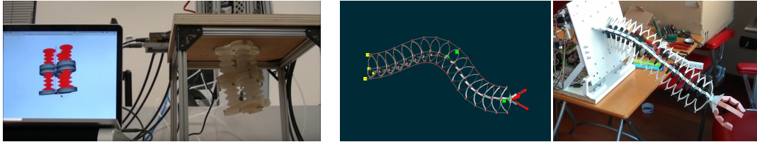
(a) Control from inverse simulation of two Fetch platforms stacked for the Soft Robotic Toolkit 2015 competition.
