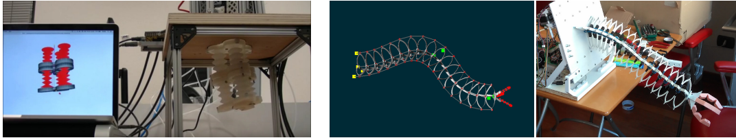
(a) Control from inverse simulation of two Fetch platforms stacked for the Soft Robotic Toolkit 2015 competition. (b) Simulation of Flexo (left) and the real robot (right).
