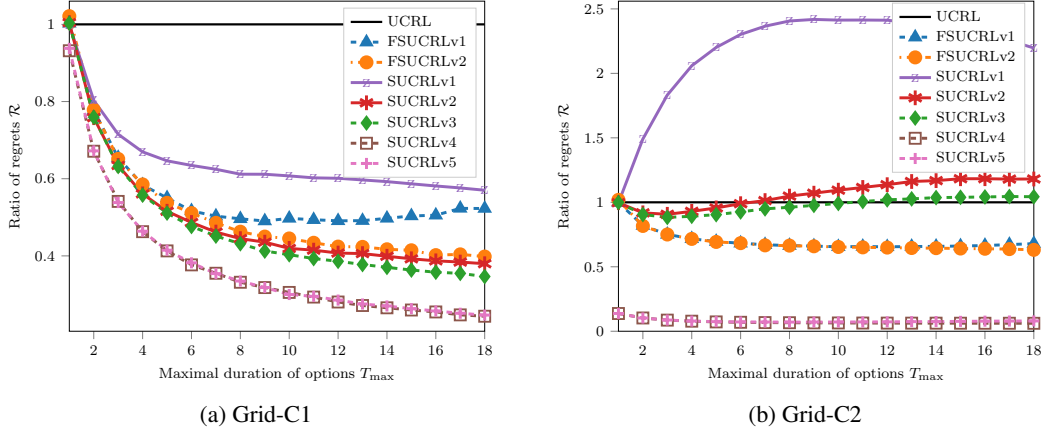
Figure 6: Empirical ratio \mathcal{R} = \Delta(\mathfrak{A}, n)/\Delta(\text{UCRL}, T_n) , with \mathfrak{A} \in \{\text{SUCRL}, \text{FSUCRL}\} and T_n = 2 \cdot 10^9 , as a function of the maximal length of options T_{\max} , when the regret term related to the estimation of the transition kernel is dominant (6a) and when the regret term related to the estimation of the reward function is dominant (6b). A detailed description of the different versions of both FSUCRL and SUCRL is reported on Table 1. We have performed 20 repetitions but there is no variability in the outcomes.
