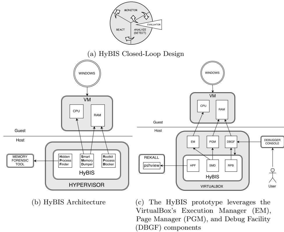
Fig. 1: HyBIS Design, Architecture, and Implementation Details
