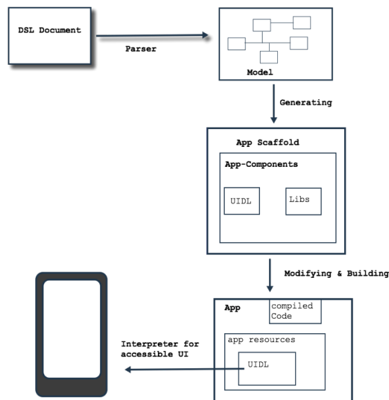
Fig. 3. Workflow from Meta-Model to Model to App Scaffold to final App.
