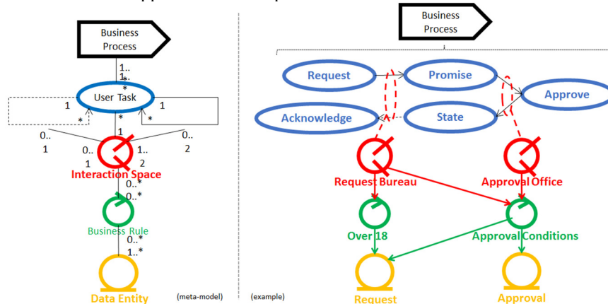
Fig. 6. Enterprise Structure meta-model and example.
