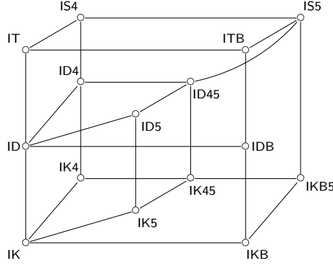
Figure 2: The intuitionistic “modal cube”
