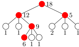
Figure 4: Example showing that a chain always wastes processors. Node labels represent their subtree computational weight. All edges have weight 10, and p = 6 . Red nodes denote subtrees' roots as determined by ASAP .
