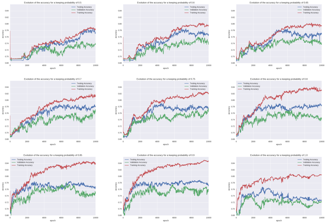
(b) Evolution of the accuracy for different Testing keeping probabilities.
