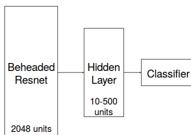
Figure 4: Architecture used for our naive approach
