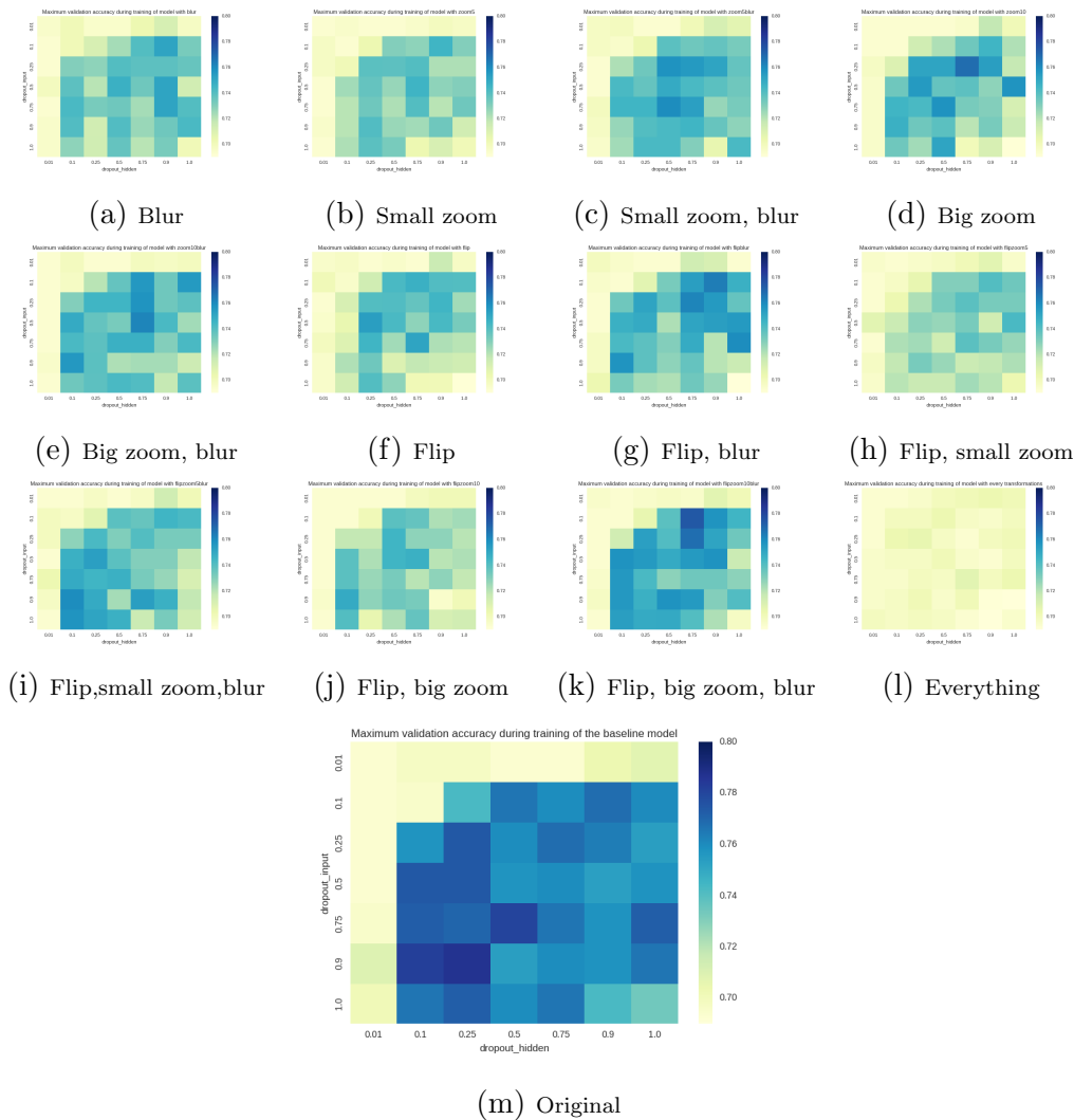
Figure 7: Results from data augmentation
