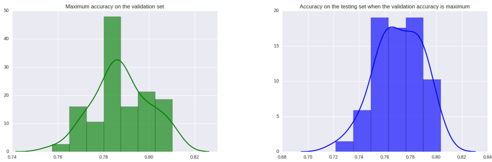
(a) Maximum validation accuracy and associated testing accuracy.
