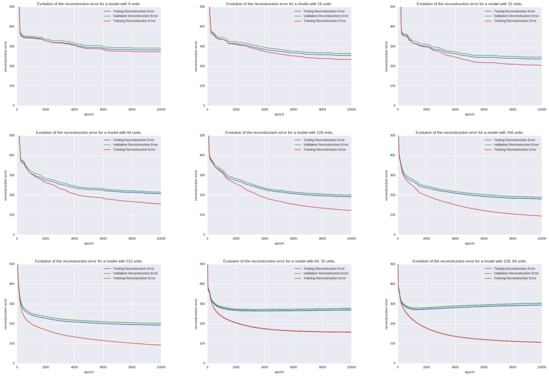
(a) Evolution of the reconstruction error for auto-encoders.
