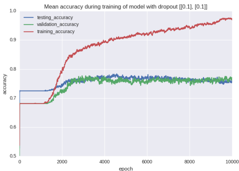
Figure 5: Example of a graph representing the training of one model
