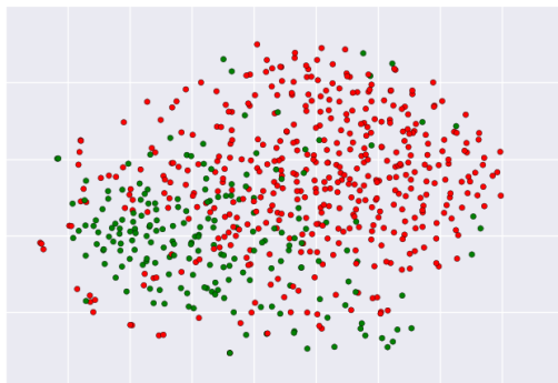
(c) TSNE of the representation from the Feed Forward approach
