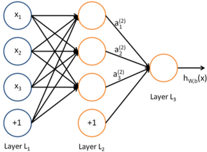
Figure 2: General architecture of a layer of a neural network. Source: Stanford.
