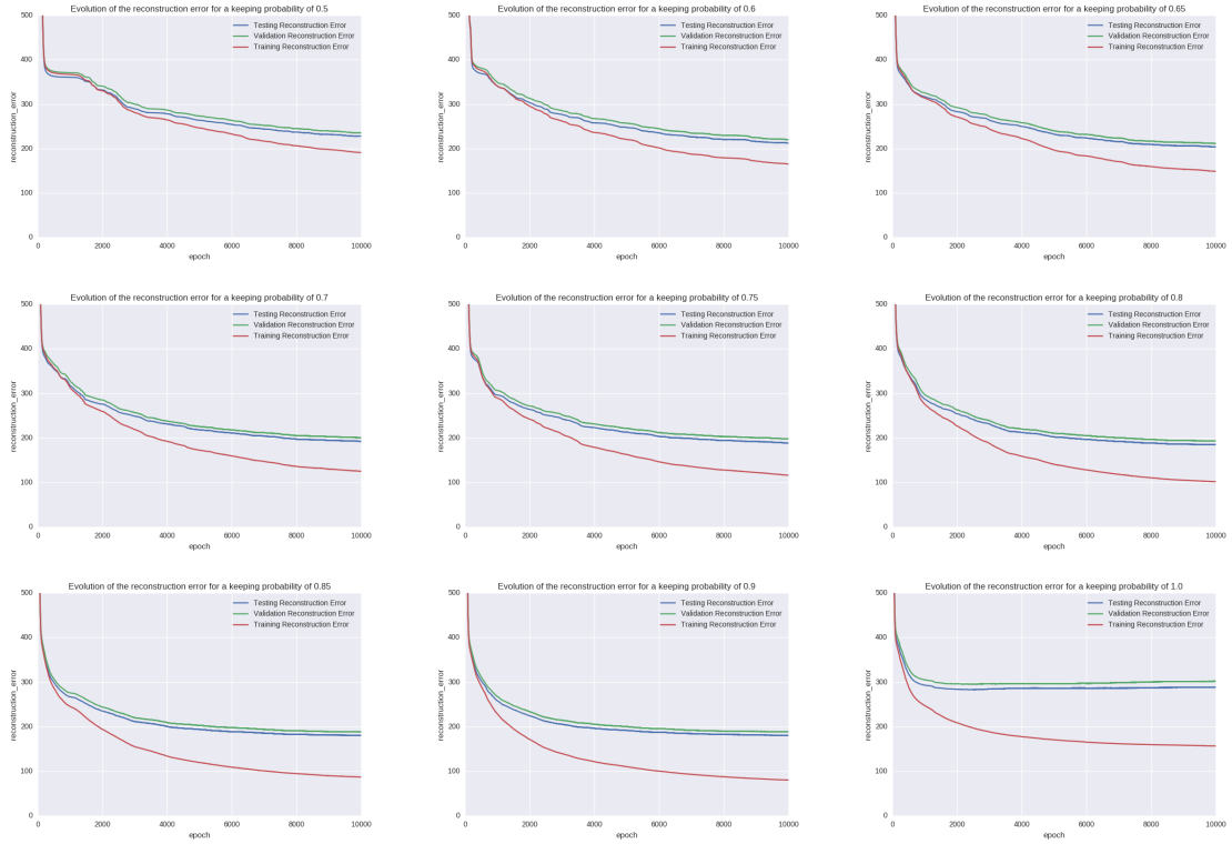
(a) Evolution of the reconstruction error for different keeping probabilities.
