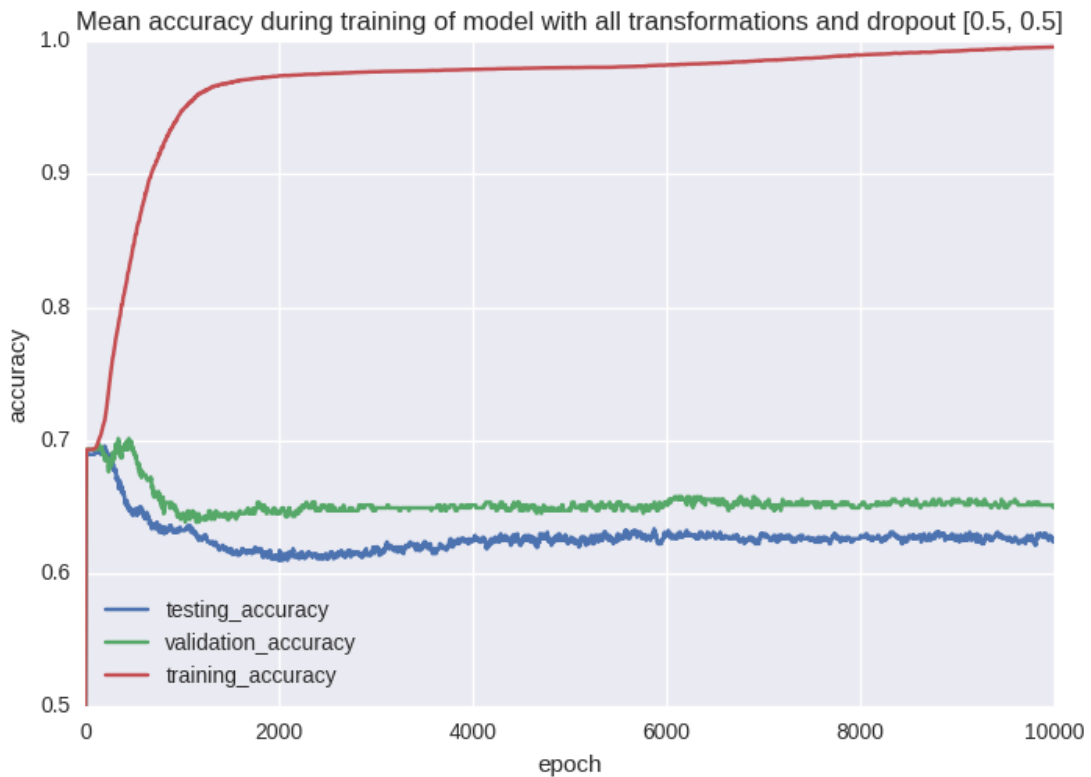
Figure 20: Evolution of the accuracies during the training of a neural network with every augmented pictures.
