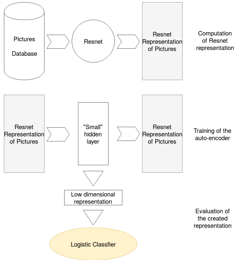
Figure 11: Schema of the approach with auto-encoders.
