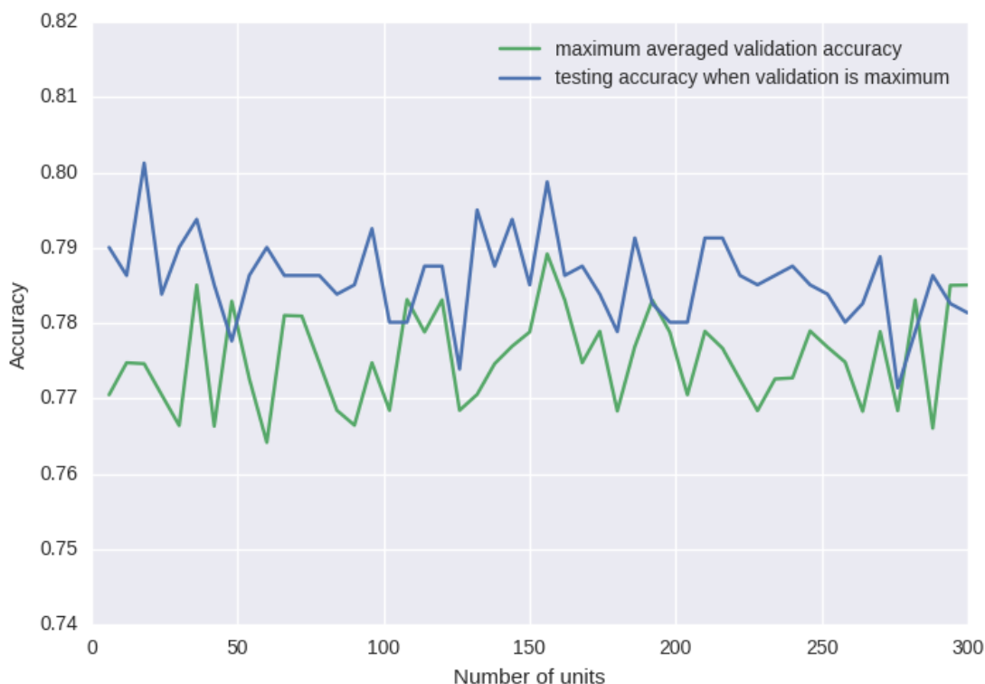
Figure 10: The evolution of maximum averaged validation accuracy and associated testing accuracy with the size of the hidden layer
