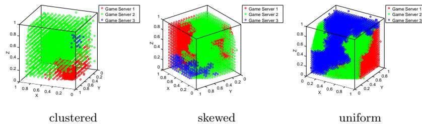
Fig. 3: Avatar Grouping ( P=10 , 3 servers, 1000 avatars)
