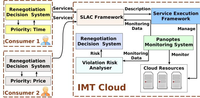
Fig. 2: Components of the use case framework.
