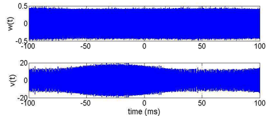
Fig. 7: vibration amplitude w(t) of the transducer (top) in closed loop; the amplitude of the voltage (bottom) vary when a user modifies his pressure on the head's surface.
