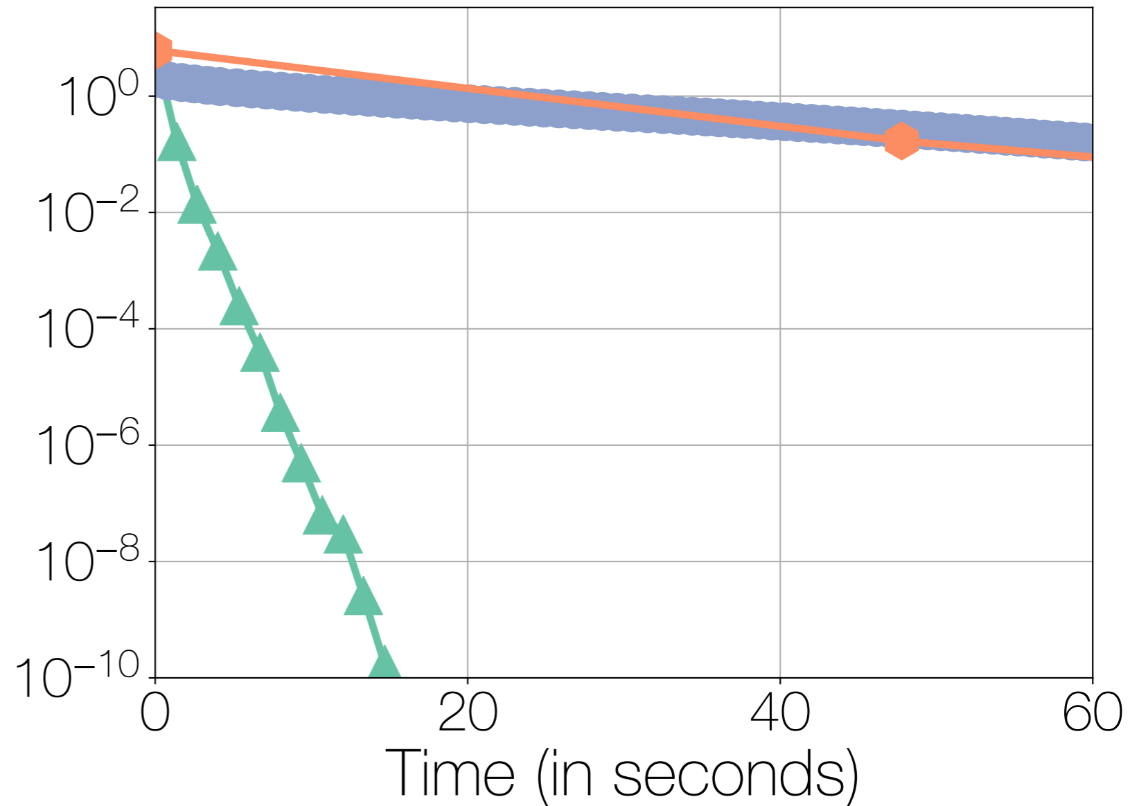
RCV1-full dataset
