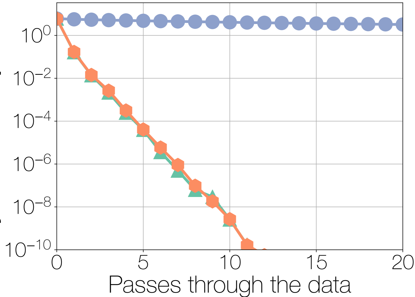
RCV1-full dataset
