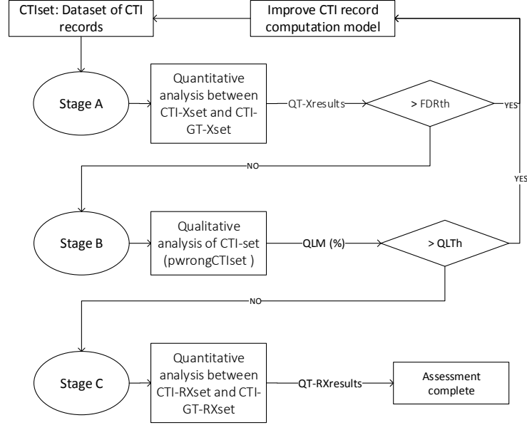
Fig. 1. Workflow of the CTI-QAF
