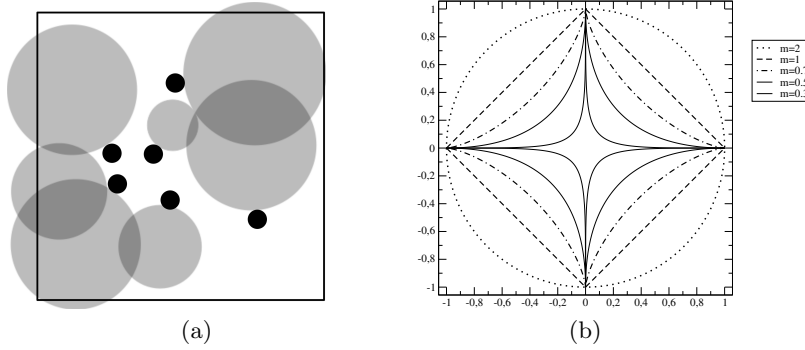
Fig. 1: (a) Example of performance V-Detector algorithm for 2-dimensional problem. Black and grey circles denotes self samples and v -detectors, respectively. (b) Unit spheres for selected L_m norms in 2D.
