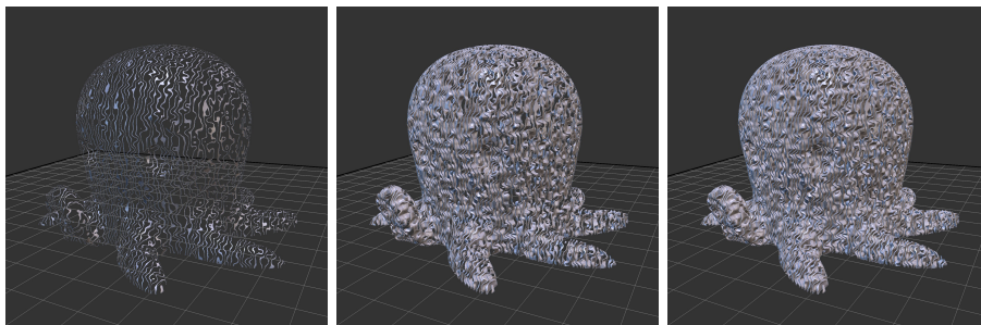
Figure 3: Gradual ray-marching on the CuteOcto model (thing:27053 by Maker-Bot). From left to right: First rendered frame, then frames after respectively 1 sec and 4 sec. Images rendered at 1016^2 resolution on a GeForce GTX 980. The ray-marching step is 10\mu m , the solid implicit is f(p) = \sin(p.x * 6.0 + 6.0 * \text{noise}(p * 3.0/4.0)) < 0.75 ? 1 : 0 , where noise is a tri-linearly interpolated random scalar field with values in [-1, 1] .
