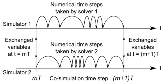
Fig. 15: Basic explicit co-simulation scheme involving two simulators
