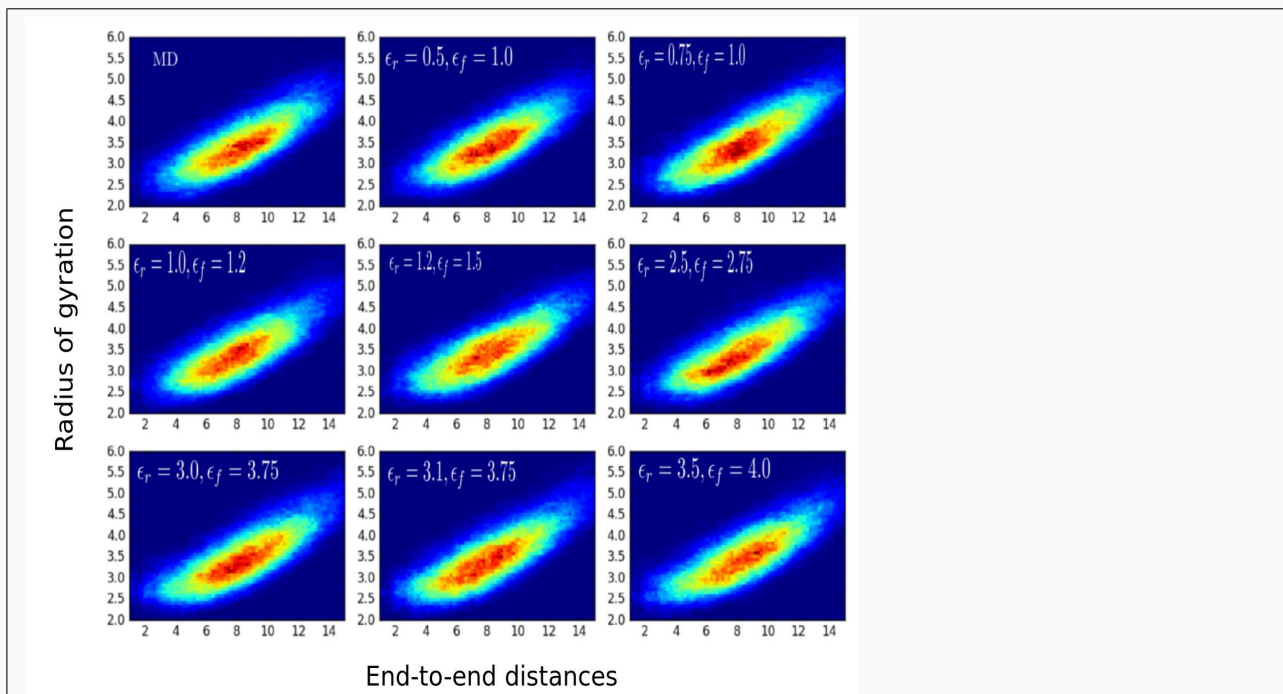
The figure represents the configuration space explore by all-atom MD and ARMD (with different restraining parameters) simulations. Adaptively switching the positional degrees of freedom on and off not only allows to perform more number of integration steps in wall clock time but also produces the unbiased and equilibrium statistics of the system.
