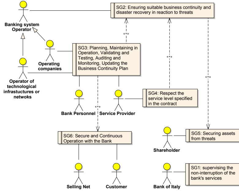
Fig. 2. Context Model: The Banking Business Continuity's Softgoals and Dependencies Diagram
