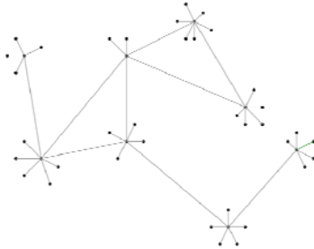
Fig. 8. Planar graph
