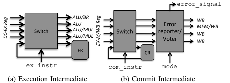
Fig. 4: Intermediate Components
