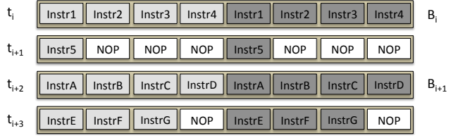
(c) Duplication of instructions with NEDA dependency analysis
