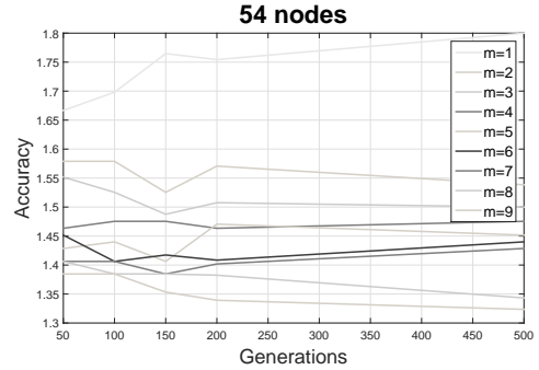
Fig. 7. Accuracy vs m (parameter of the heuristic algorithm).
