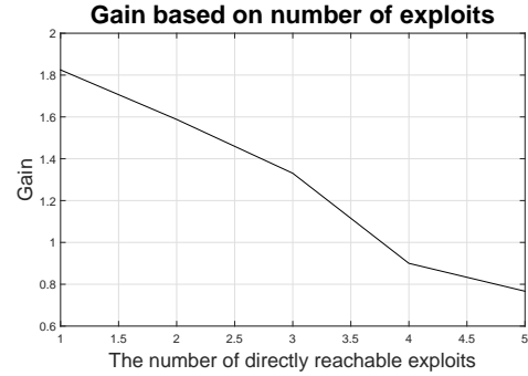
Fig. 11. Average gain based on directly reachable vulnerabilities.
