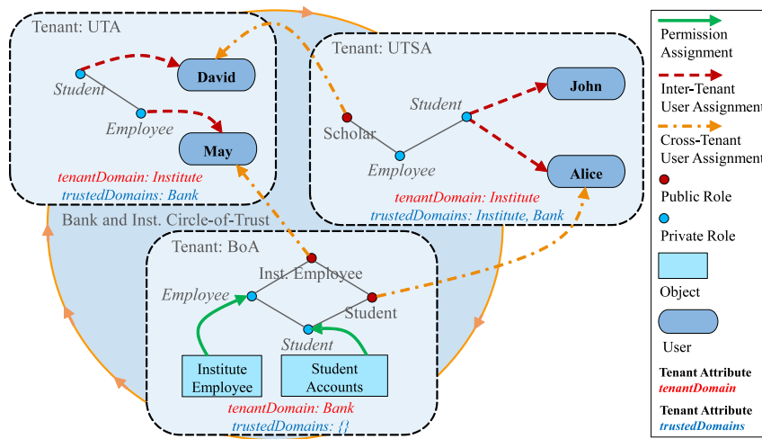
Fig. 7: Example of a Multi-Tenant RABAC c Heterogeneous Circle-of-Trust.
