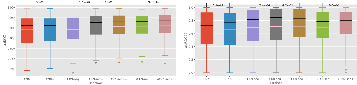
Figure 3: Performance comparison on small-scale datasets (top: DeepBind’s datasets, bottom: SCOP 1.67); CKN-seq+ (respectively uCKN-seq+) represents training CKN-seq (respectively uCKN-seq) with perturbation while CKN-seq++ means the hybrid model introduced in section 2.3 that combines supervised and unsupervised variants: all the models use 128 convolutional filters except that unsupervised CKN-seq (uCKN-seq) and uCKN-seq+ use 4096 filters for DeepBind’s dataset and 8192 for SCOP 1.67. The perturbation amount used in CKN-seq+, uCKN-seq+ and CKN-seq++ are respectively 0.2, 0.1 and 0.2 (0.3 for SCOP 1.67) for both tasks.
