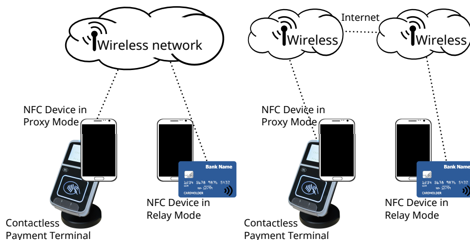
Figure 1. Setup 1: Simple Relay Attack Figure 2. Setup 2: Internet Relay Attack Setup
