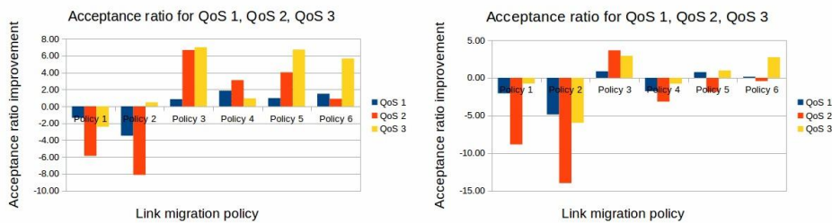
Fig. 1. Improvements (%) for HS (LEFT) and FA (RIGHT) embedding algorithms
