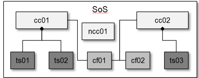
Figure 3. Architecture with connection (e.g. \text{cc01} - \text{cf01} ) and containment (e.g. \text{cc01} - \text{ts01} ) relations.
