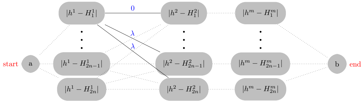
Figure 3: Graph that represents the optimization problem of equation (1). An optimal solution for (s_1, \dots, s_p) is found by finding the shortest path from node a to node b . We assume that there are n individuals in the source populations resulting in 2n haplotypes denoted by (H_1, \dots, H_{2n}) . The value (0 or 1) of the i^{\text{th}} haplotype at the j^{\text{th}} SNP is denoted by H_i^j . A vector (s_1, \dots, s_p) describes the sequence of haplotype labels from which the haplotype h of an admixed individual can be approximated. For the j^{\text{th}} SNP in the data set, s_j = k if haplotype h results from a copy of haplotype H_k .
