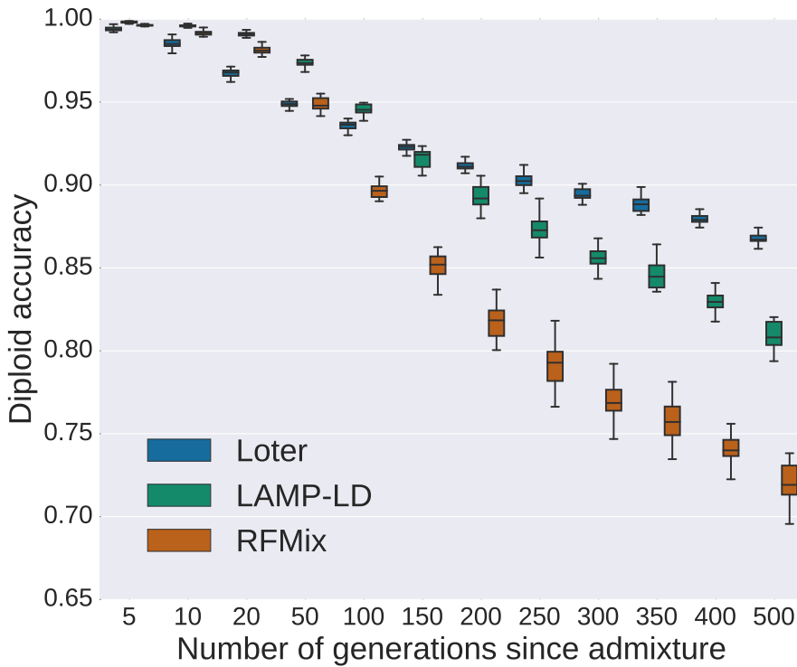
Figure 4: Diploid accuracy obtained with LAMP-LD, Loter, and RFMix for simulated admixed human individuals as a function of the time since admixture occurred. Admixed individuals are simulated by constructing their genomes from a mosaic of true African (YRI) and European (CEU) haplotypes (International HapMap 3 Consortium et al. 2010). For performing simulations, true haplotypes are obtained using trio information. For local ancestry inference, haplotypes are obtained with Beagle using individuals that are not used for simulating admixed individuals. For each value of the number of generations since admixture, 20 sets of 48 admixed individuals are generated. Boxplots show the distribution of the 20 values for the mean diploid accuracy.
