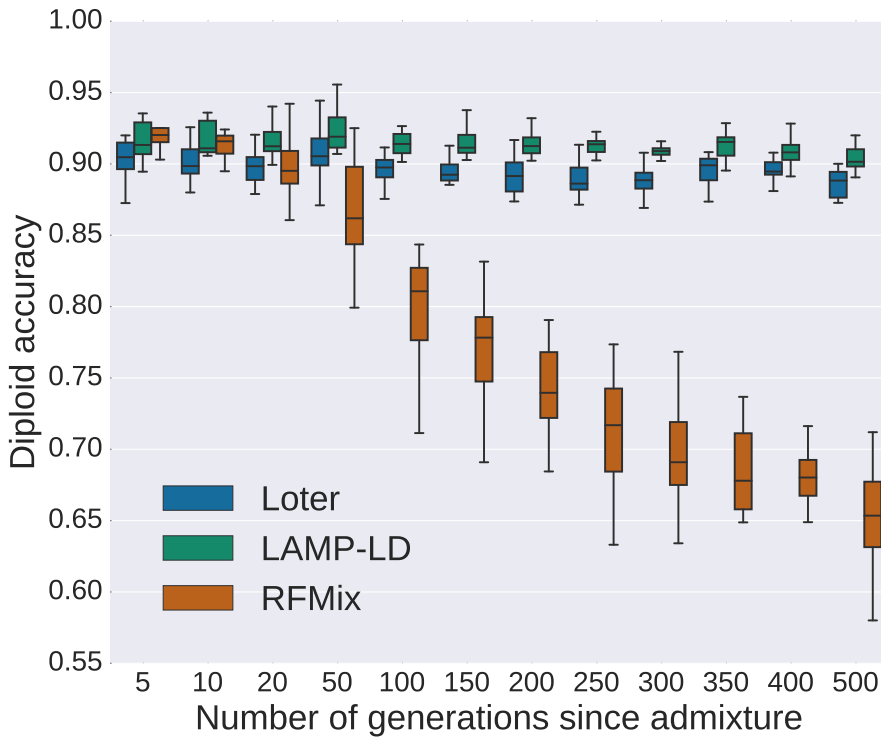
Figure 5: Diploid accuracy obtained with LAMP-LD, Loter, and RFMix for simulated admixed Populus individuals as a function of the time since admixture occurred. Admixed individuals are simulated by constructing their genomes from a mosaic of Populus trichocarpa and Populus balsamifera individuals. Individuals are phased using Beagle and two different sets of individuals are used for performing simulations and inference. For each value of the number of generations since admixture, 20 sets of 20 admixed individuals are generated. Boxplots show the distribution of the 20 values for the mean diploid accuracy.
