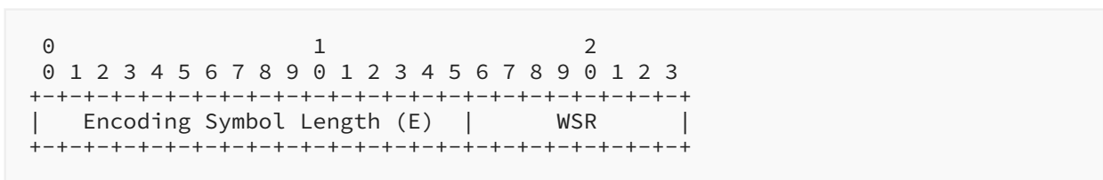
Figure 4: FSSI Encoding Format
