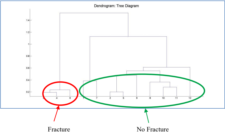
Fig. 4. Both FFT and Wavelet Decomposed Coefficients produced the same results by the dendrogram.
