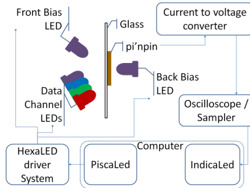
Fig. 4. Sensor and LED relative positions and equipment
