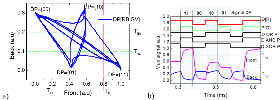
Fig. 12. a) Scatter graph of the resulting Back and Front bias signals of Fig. 11 and b) detail of Fig. 11, contains all 4 combinations of two digital signals, front and back are the interaction of two signals D,P, and the OR, AND, XOR signals represent the expected output.
