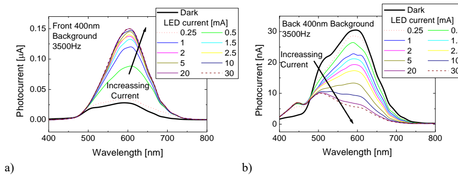
Fig. 2. Sensor photocurrent output using optical bias wavelength of 400 nm at the a) front and b) back sides.
