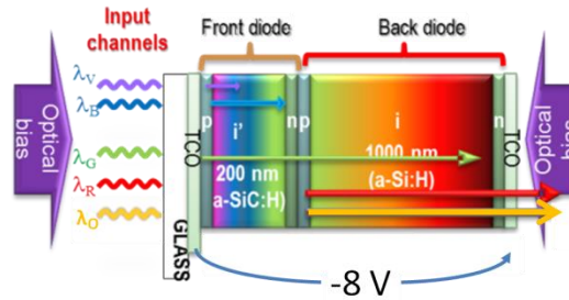
Fig. 1. Sensor structure and operation
