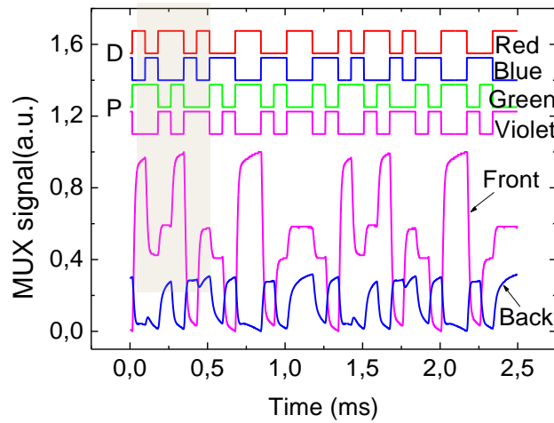
Fig. 11. Result of the interaction of two digital light signals D[Red, Blue] and P[Green, Violet]
