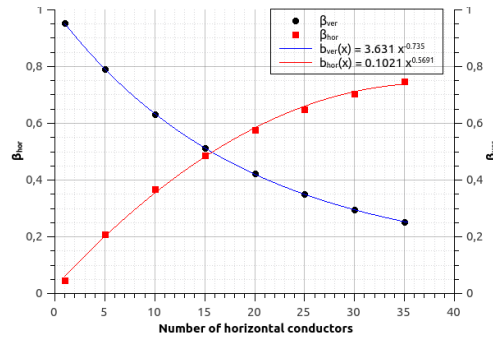
Fig. 3. Posynomial form function for the horizontal and the vertical heat ow ratio calculation.
