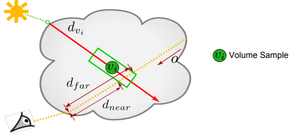
Fig. 5. Single scattering: we add the contributions from all volume samples whose OOB is intersected by the camera ray.
