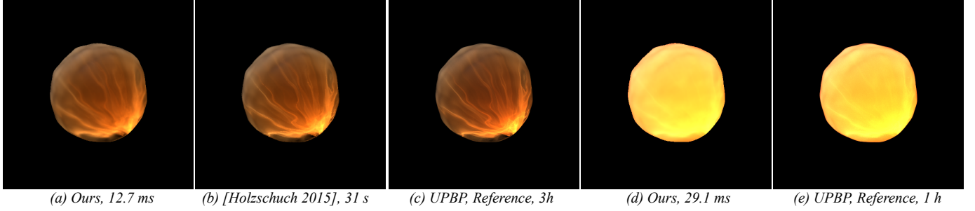
Fig. 13. Individual component validation on the Bumpy Sphere scene, interactive GPU implementation. (a) to (c): single scattering only. (d), (e): full solution.
