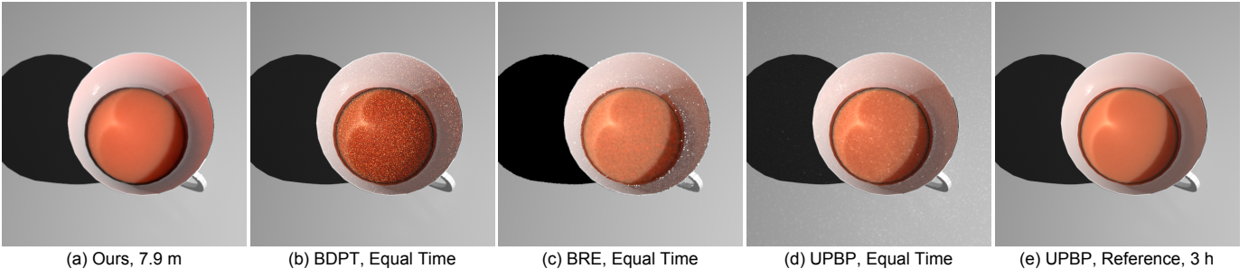
Fig. 18. Inside Material: bumpy sphere material with g = 0.0 , and scale = 5. Note the caustics caused by light reflecting on the glossy cup surface. For this material, with a large albedo and a small mean free path, multiple scattering effects dominate. Outside Material: Phong model, specular exponent: 800.
