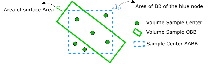
Fig. 4. Density factor: for each volume sample, we compute the ratio between the area of its leaf node A_v and the area S_v around the surface sample at the origin of the ray. A_v is larger in low density areas, smaller in high-density regions.
