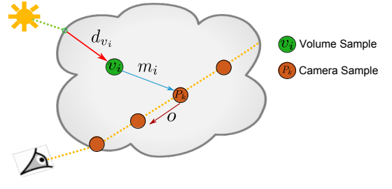
Fig. 6. Double scattering: we extract a tree-cut of volume samples and compute double scattering from each node of this tree-cut.
