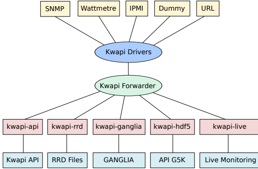
Figure 3: KWAPI architecture [46].
