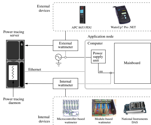
Figure 8: Architecture of PML LIB .
