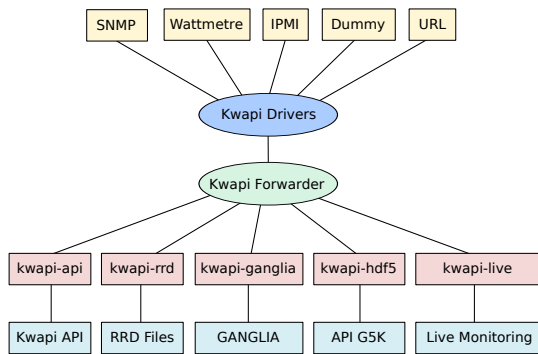
Figure 3: KWAPI architecture [46].
