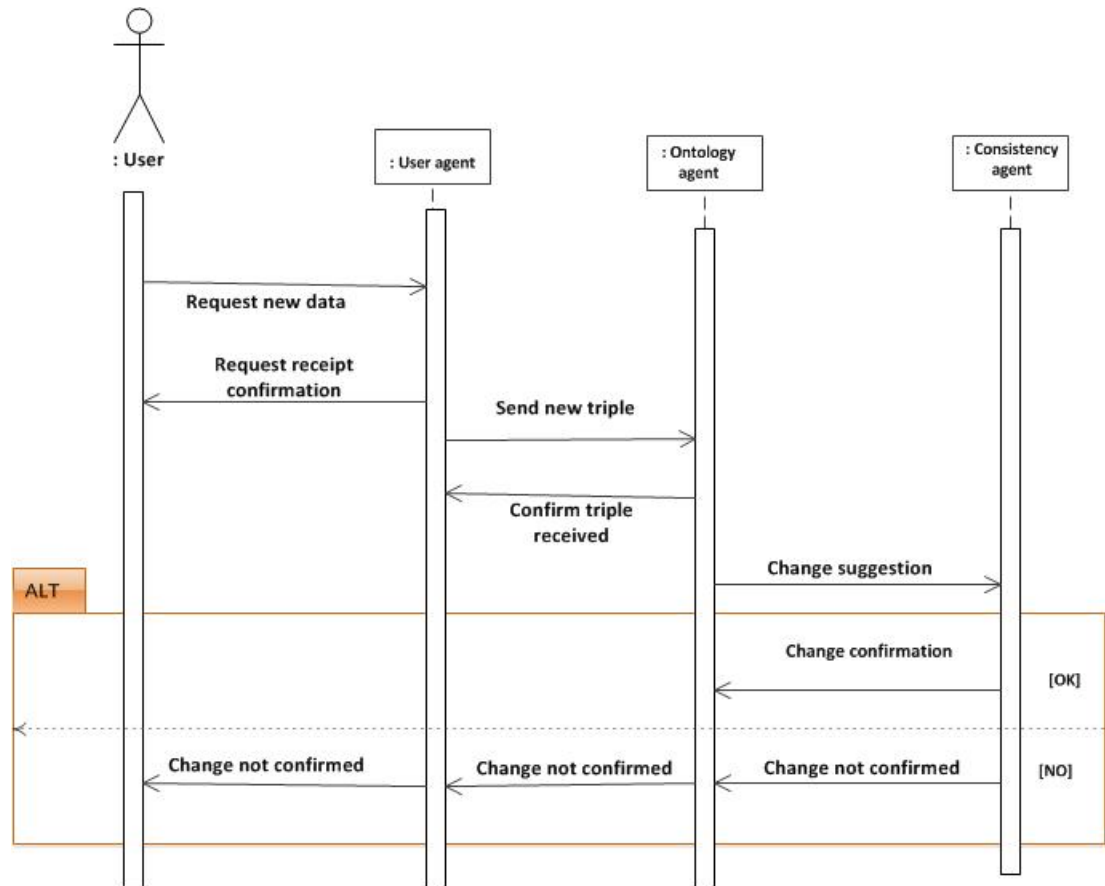
Fig. 3. Sequence diagram that models inter-agent communication.
