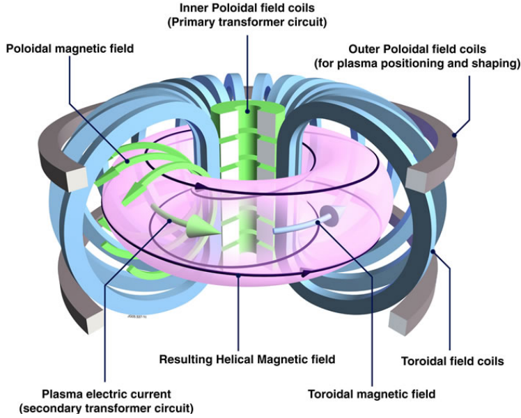
Fig. 1. Schematic representation of a tokamak
