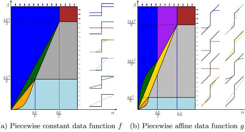
Fig. 1: Exact solutions for the L^2 - \text{TVL}_{\alpha,\beta}^\infty one dimensional denoising problem
