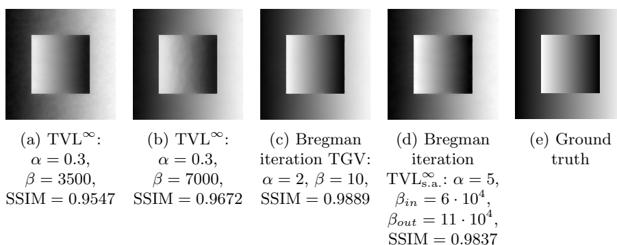
Fig. 5: \text{TVL}^\infty reconstructions for different values of \beta . The best result is obtained by spatially varying \beta , setting it inversely proportional to the gradient, where we obtain a similar result to the TGV one
