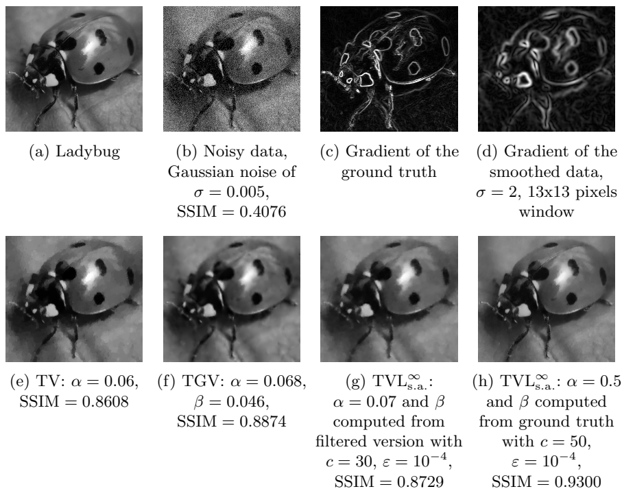
Fig. 6: Best reconstruction of the “Ladybug” in terms of SSIM using TV, TVG and spatially adapted \text{TVL}^{\infty} regularisation. The \beta for the latter is computed both from the filtered (Figure 6g) and the ground truth image (Figure 6h)
