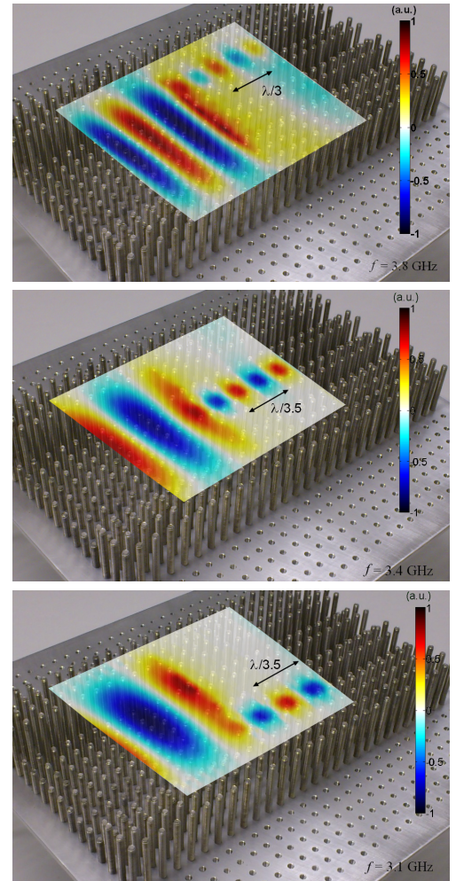
FIG. 6: Electric fields scanned above the structure at three frequencies chosen respectively in the red ( f = 3:1 GHz), green ( f = 3:4 GHz) and blue ( f = 3:8 GHz) frequency range [f_c^-; f_c^+] .
