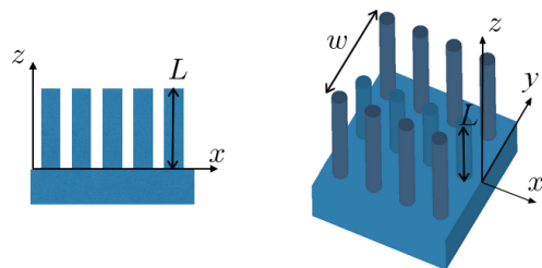
FIG. 1: (a) 2D geometry of metallic layers between a ground plane and the air, spoof plasmons can propagate according to (1), (b) 3D geometry of a structured waveguide of width w , guided modes can propagate according to Eq. (6).
