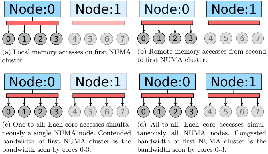
Fig. 2: Modeled memory access patterns.
