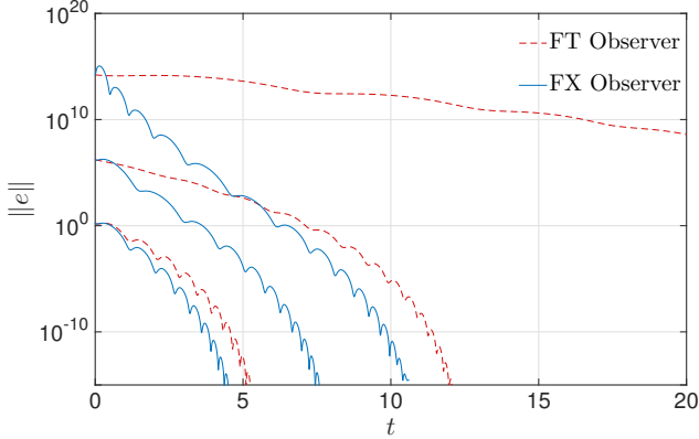
Fig. 3. Simulation plot of \|e\| for the FT and FX observers applied to the linearized plant for three different IC x(0) = (0, 1, \frac{\pi}{4}, 0) , x(0) = 10^3(0, 1, \frac{\pi}{4}, 0) , x(0) = 10^7(0, 1, \frac{\pi}{4}, 0) and K_p = 5 .
