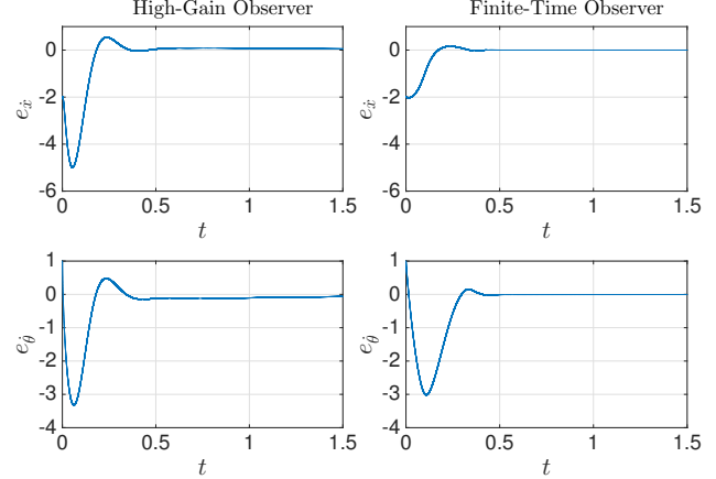
Fig. 1. Simulation plots of e_x and e_\theta for the HG and FT observers applied to the nonlinear plant with IC x(0) = (0, -2, \frac{\pi}{4}, 1) and K_p = 10 .
