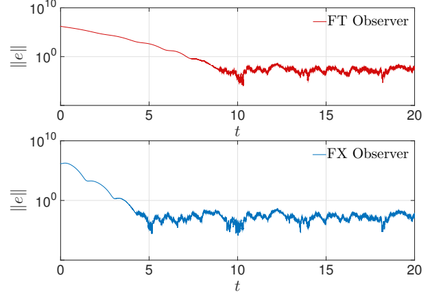
Fig. 4. Simulation plot of \|e\| for the FT and FX observers with measurement band limited noise to the linearized plant with IC x(0) = 10^3(0, 1, \frac{\pi}{4}, 0) and K_p = 5 .
