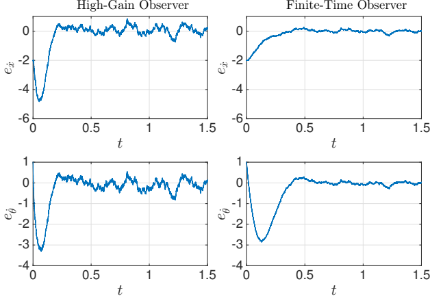
Fig. 2. Simulation plots of e_{\hat{x}} and e_{\hat{\theta}} for the HG and FT observers with a band-limited white noise in the measurements.
