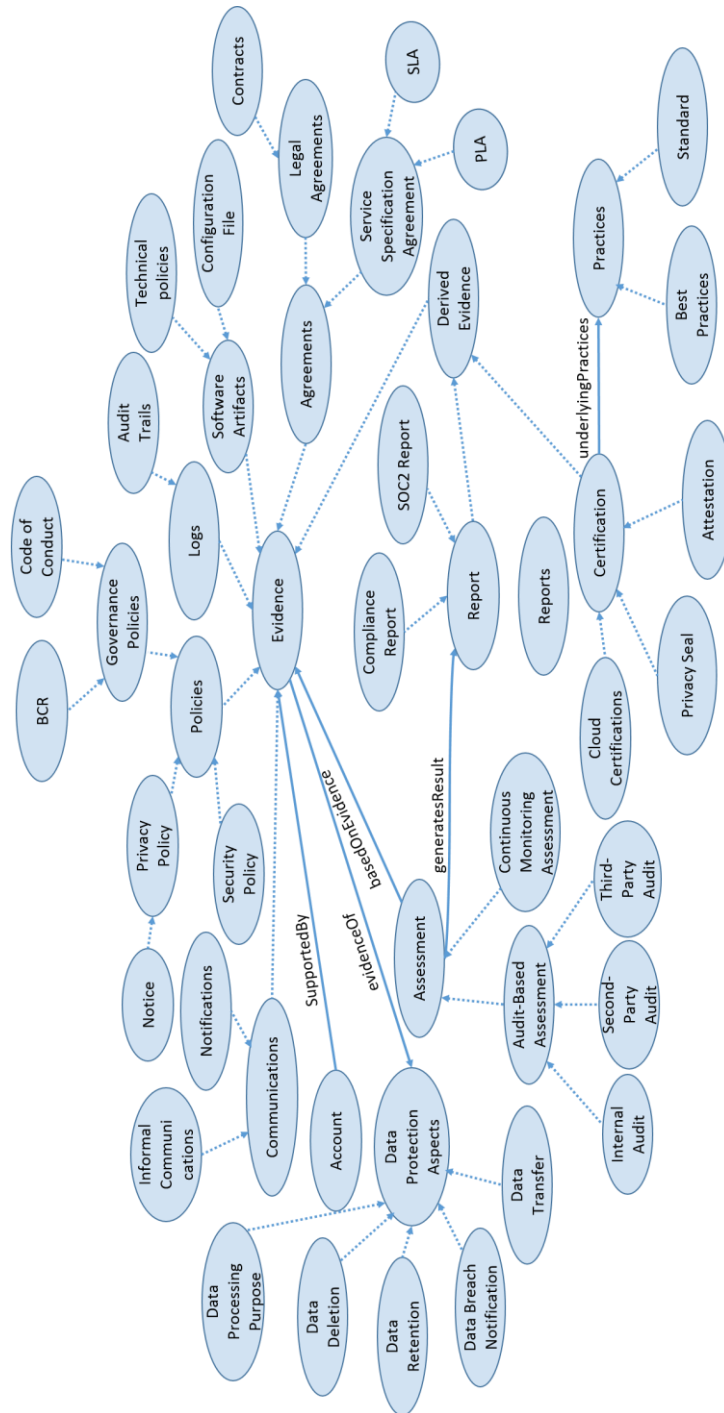
Fig. 2. Evidence Ontology
