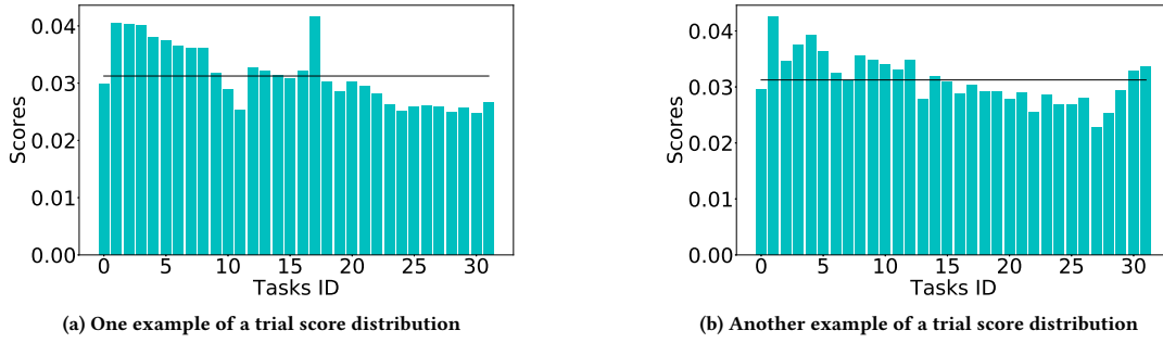
Figure 1: Examples of trial score distributions generated by the simulation procedure for a tuple of task sets (S, Q) , with |S| = 16 and |Q| = 32 , in a cluster with 256 nodes. The black horizontal line represents the mean \frac{1}{|Q|} = \frac{1}{32} = 0.031 .
