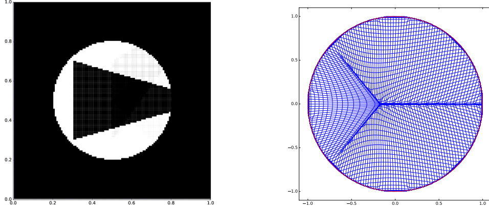
Figure 12: Left: Source density f . Right: Corresponding optimal map deformation of the grid.
