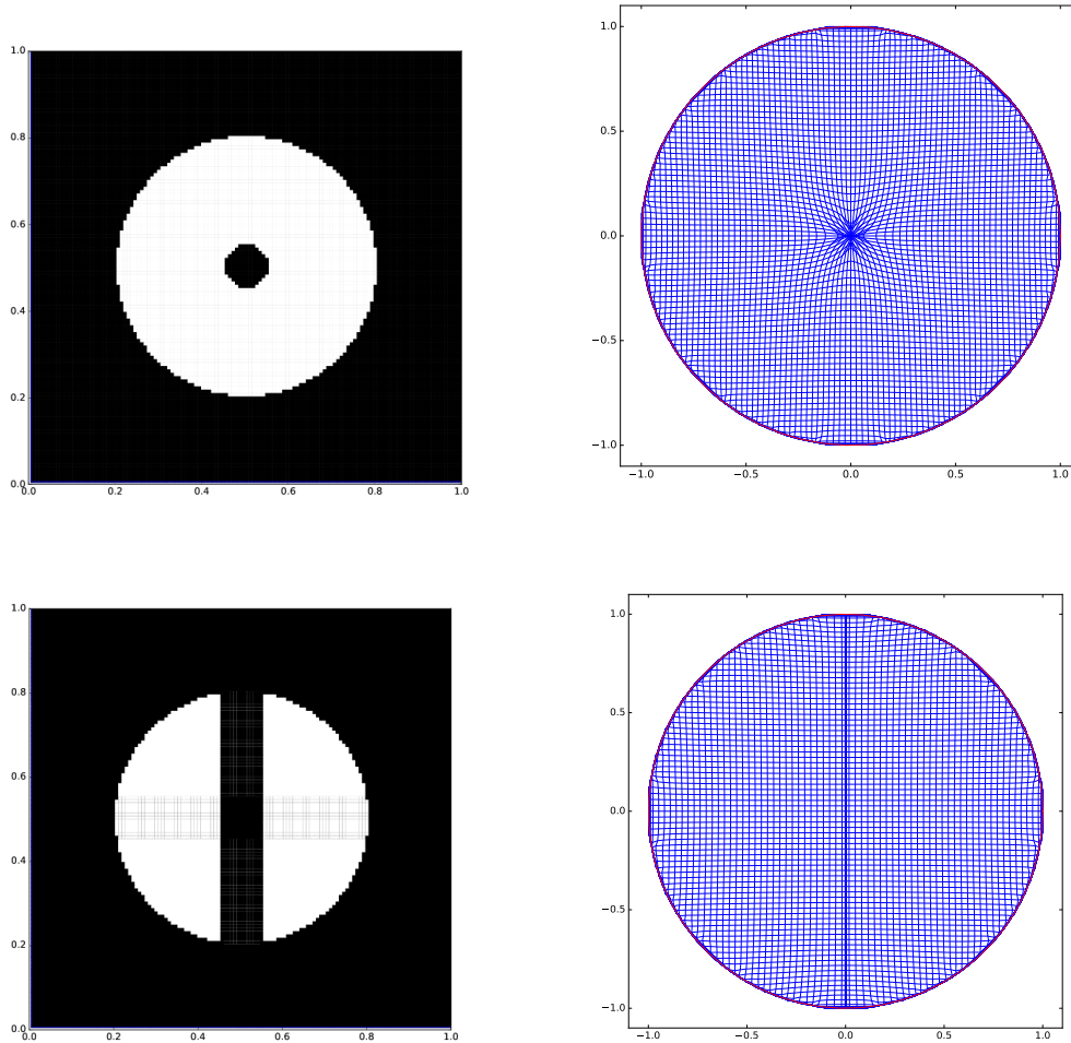
Figure 10: Left column: Source density f . Right column: Corresponding optimal map deformation of the grid.
