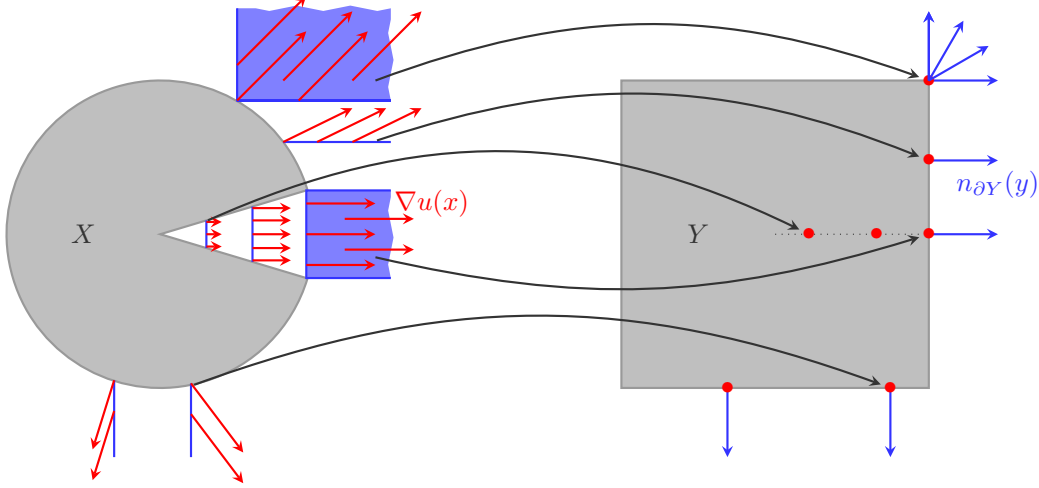
Figure 1: Illustration of Proposition 3.5 showing the correspondence between gradients (red) and their support (blue) in source space and target space. The connected blue regions in the source space represent points which are mapped to the same gradient value (in red).
