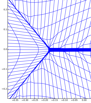
Figure 13: Zoom of Figure 12, Right.
