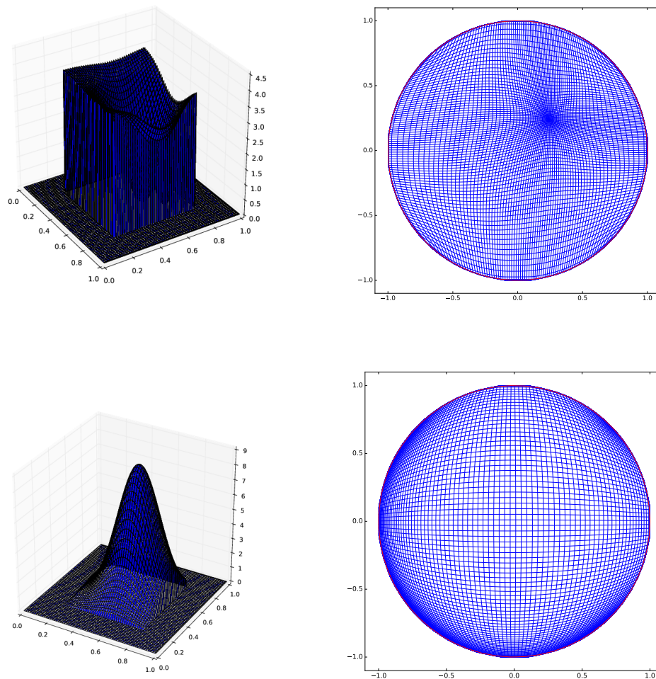
Figure 7: Left column: Source density f . Right column: Corresponding optimal map deformation of the grid.
