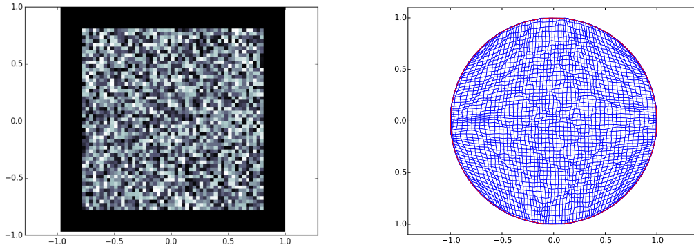
Figure 8: Left: Source density f . Right: Corresponding optimal map deformation of the grid.
