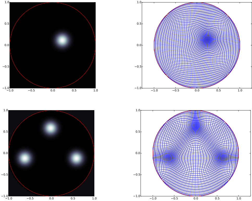
Figure 9: Left: Target density g . The boundary of the target is the red circle. Right: Corresponding optimal map deformation of the grid.
