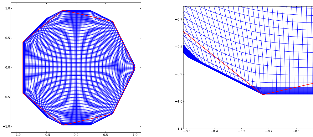
Figure 4: Left: Mapping a square to heptagon, Stencil width = 2. Right: zoom.
