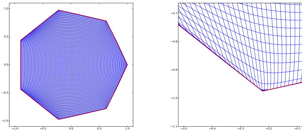
Figure 6: Left: Mapping a square to heptagon, Stencil width = 16. Right: zoom.
