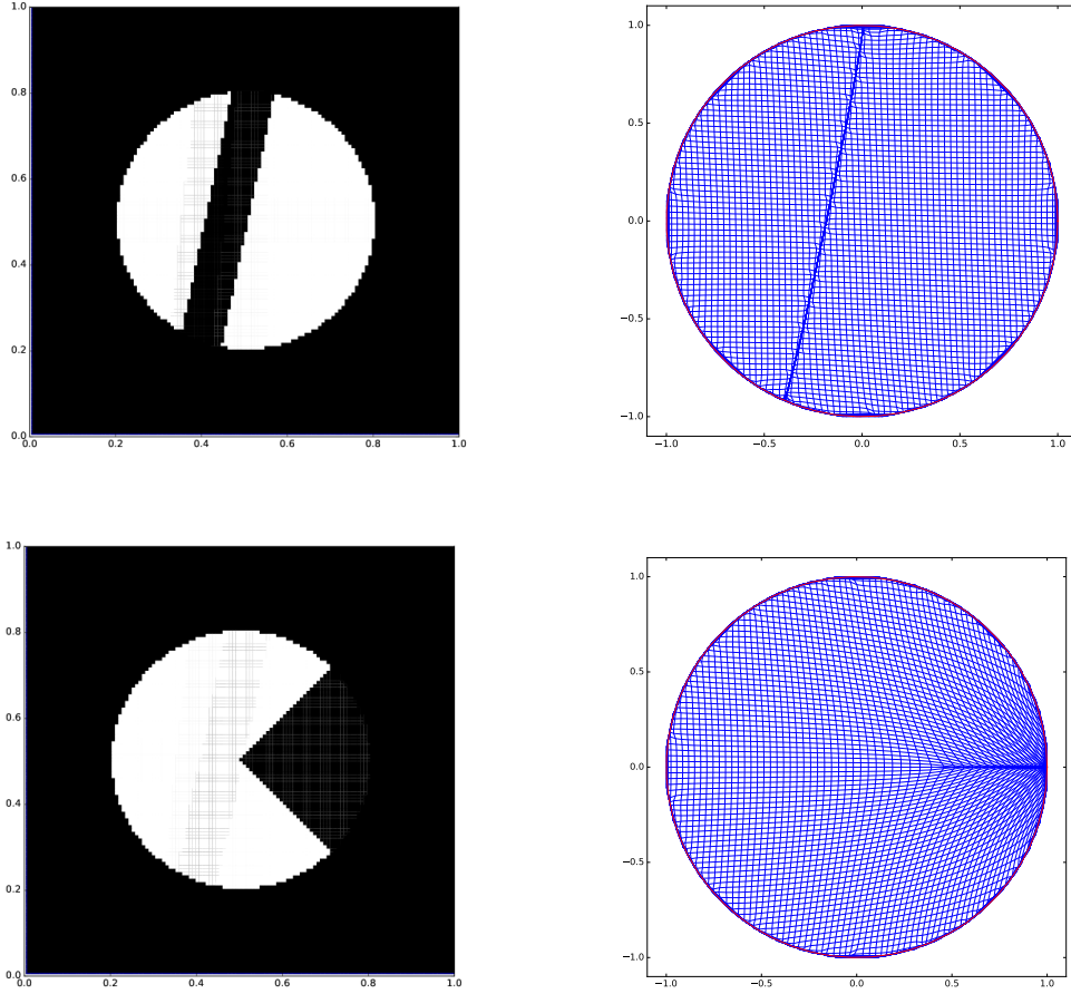
Figure 8: Left column: Source density f . Right column: Corresponding optimal map deformation of the grid.
