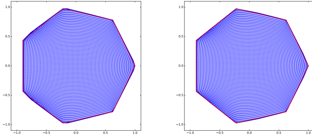
Figure 4: Mapping a square to heptagon. Left: stencil width = 4. Right: stencil width = 8.
