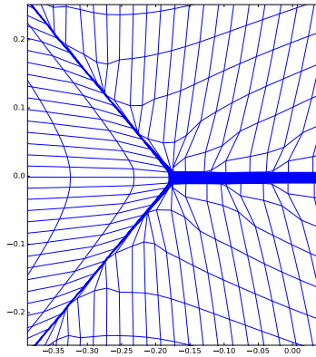
Figure 10: Zoom of Figure 9, Right.
