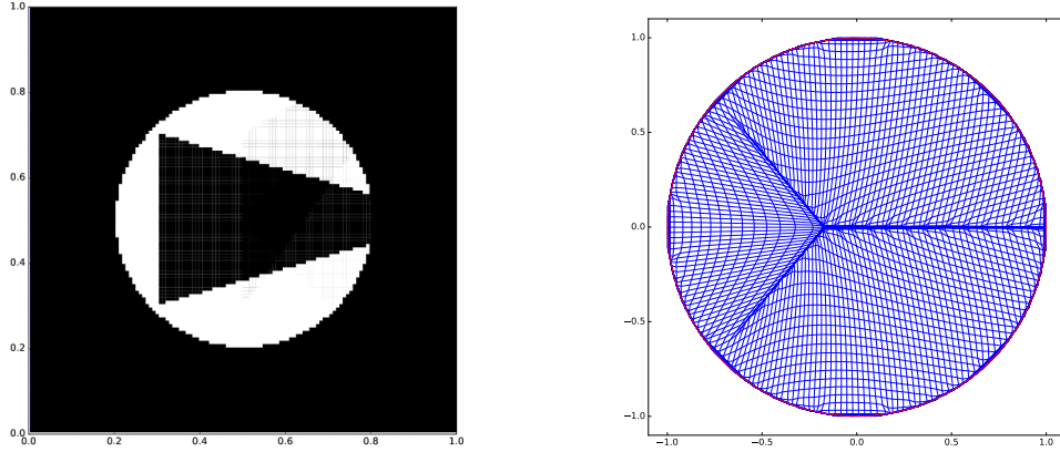
Figure 9: Left: Source density f . Right: Corresponding optimal map deformation of the grid.
