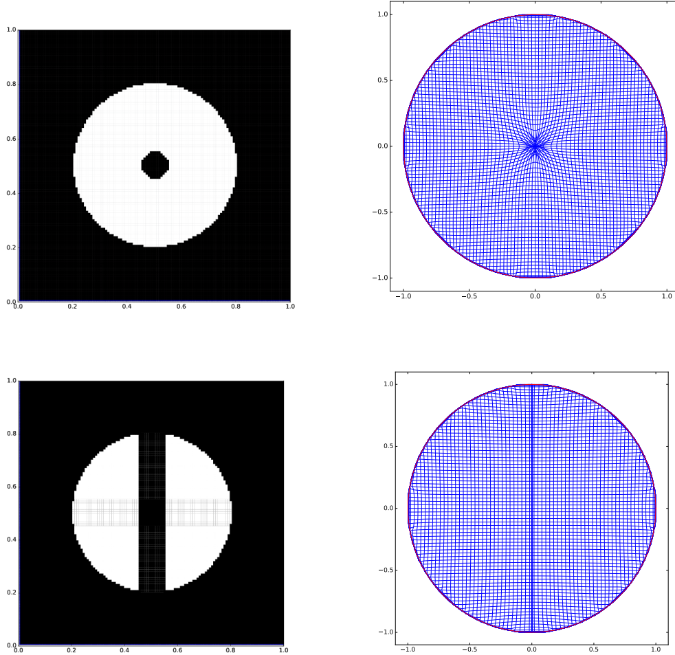
Figure 7: Left column: Source density f . Right column: Corresponding optimal map deformation of the grid.
