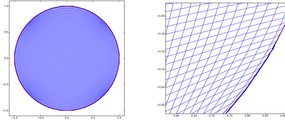
Figure 2: Left: Map deformation of the cartesian grid for square to ball test case. Right: Zoom of the Map deformation of the cartesian grid (test case to see D \setminus X mapped to \partial Y . Only the position of the grid points is really significant...)
