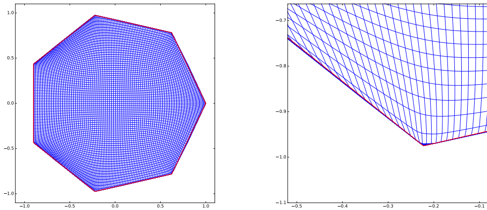
Figure 5: Left: Mapping a square to heptagon, Stencil width = 16. Right: zoom.
