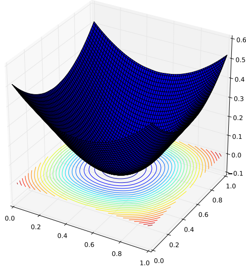
Figure 1: Surf and contour plot of the potential \tilde{u} when mapping X = [0.2, 0.8]^2 to Y = B(0, 1) (with uniform densities). The potential is smooth and affine in D \setminus X .
