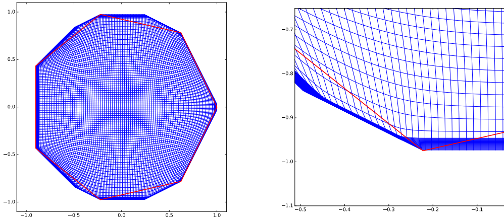
Figure 3: Left: Mapping a square to heptagon, Stencil width = 2. Right: zoom.
