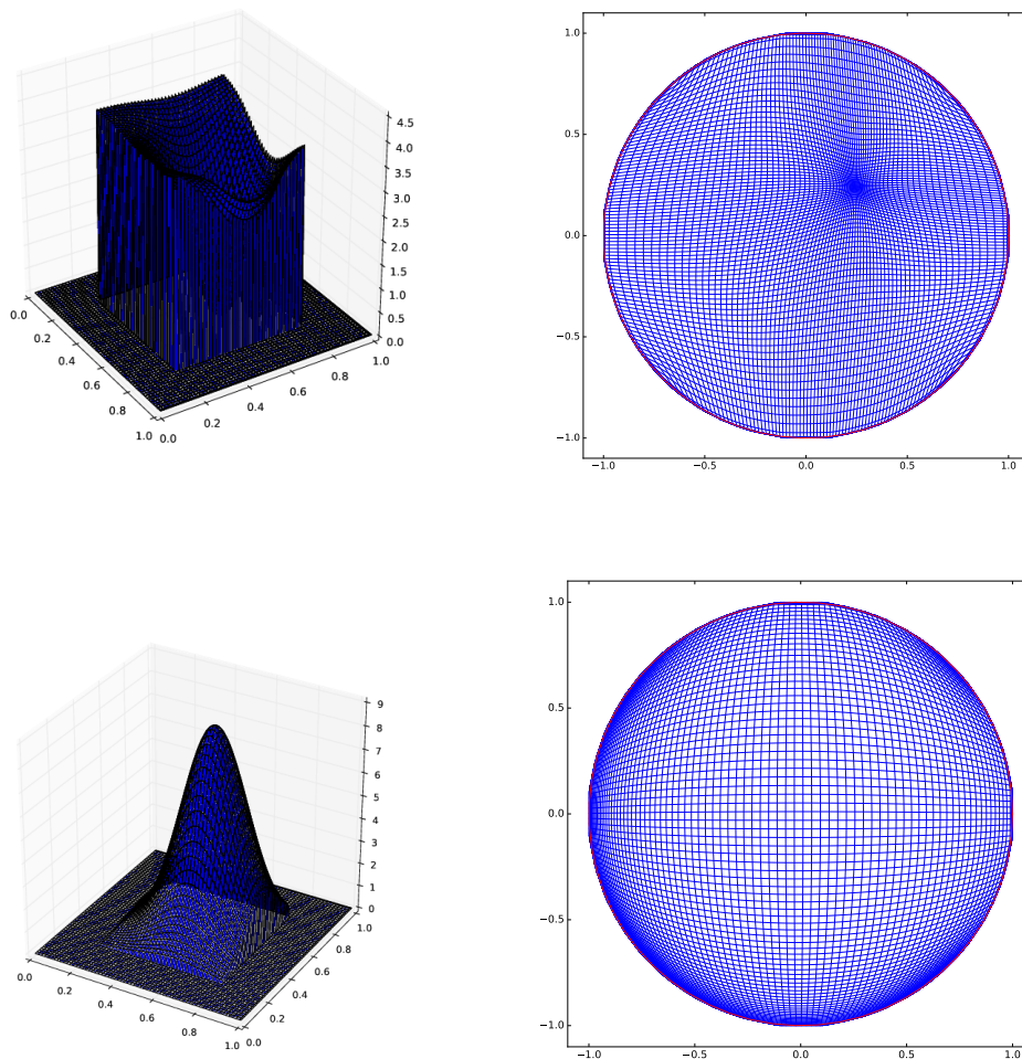
Figure 6: Left column: Source density f . Right column: Corresponding optimal map deformation of the grid.
