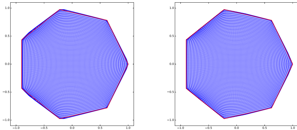
Figure 6: Mapping a square to heptagon. Left: stencil width = 4. Right: stencil width = 8.
