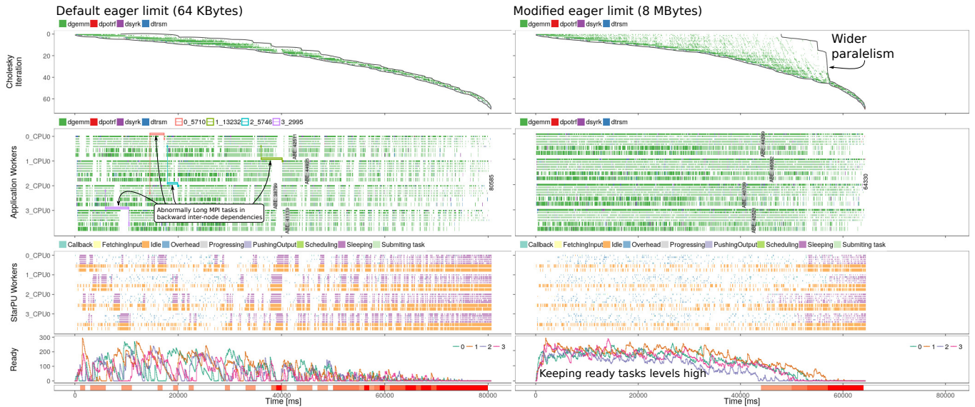
FIGURE 18 Cholesky execution using a squared matrix of 67,200, with squared tiles of 960 with four identical nodes, each one with 2 GPUs and 5 cores, LWS scheduler. The left image shows the behavior when the application executes with the default eager limit, obtaining a total makespan of \approx 80 s. It is annotated with four inter-node backward MPI dependencies showing abnormal long times. The right image (same scale) shows an unchanged case but with a larger eager limit, for a makespan of \approx 64 s (performance gain of 20%).
